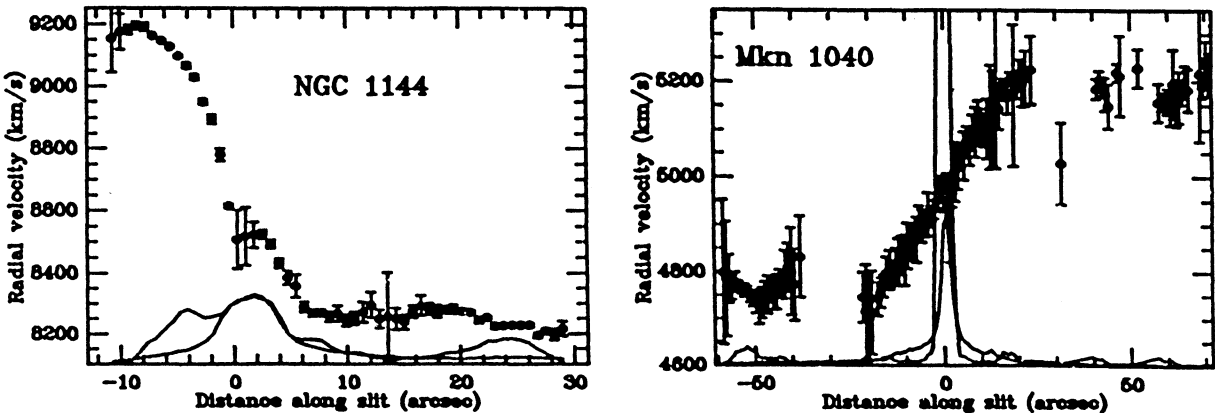
Fig. 2 – Rotation curves for paired Seyferts, showing large areas of solid-body rotation.
