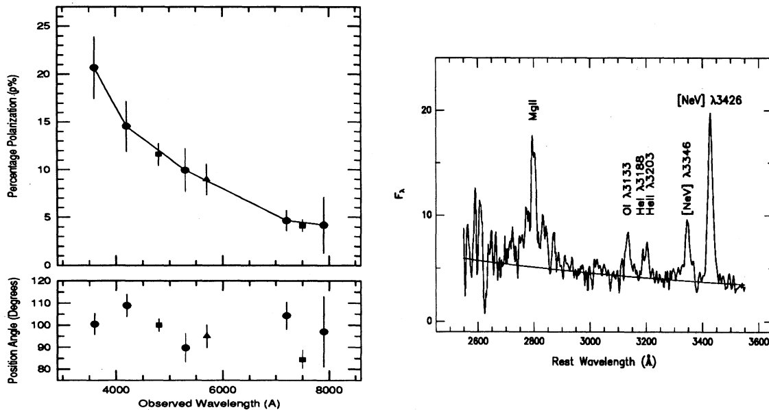
Figure 1 — Left: Observed broad band, optical linear polarization: circles represent measurements made with the UBVRI filters, the triangle represents the “open” filter observations, and the squares represent the observations made with the \text{CuSO}_4 and RG630 filters. The observed polarizations have been bias-corrected using the prescription of Wardle & Kronberg (1974). Error bars are 1\sigma (pure photon-counting statistics). The position angle errors are 1\sigma errors except for the I -band, which are not well-defined because of the low significance of the measurement. These errors do not include the \pm 2^\circ absolute position angle calibration error. Right: Observed total flux spectrum showing the broad MgII emission line. The flux densities are in arbitrary units. A fitted power law continuum is shown.
