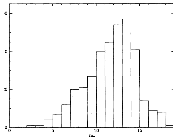
g. 5. The distribution of apparent visual magnitudes of ie secondaries.
