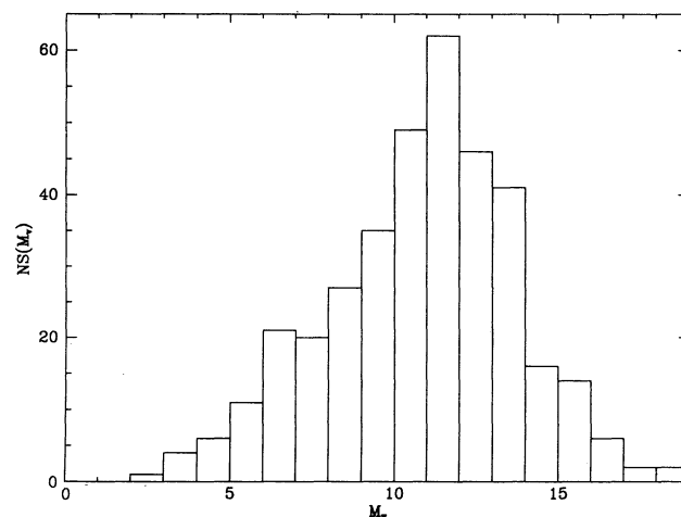
Fig. 7. The distribution of absolute visual magnitudes of the secondaries.
