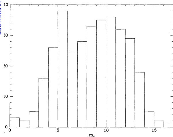
g. 4. The distribution of apparent visual magnitudes of e primaries.
