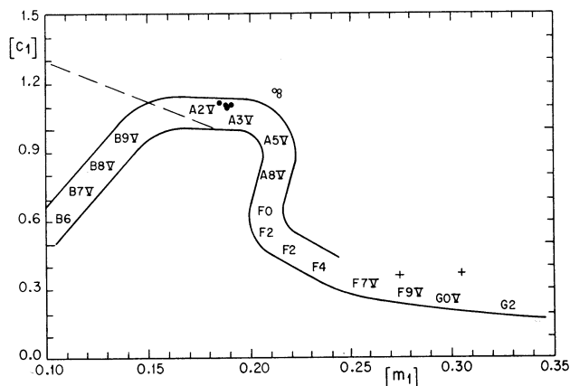
Fig. 4. [m_1] - [c_1] diagram. It defines three main spectral regions as well as the membership of the stars to the main sequence. Filled circles correspond to the nebular object; open circles to the reference star C1 and + sign to the possible eclipsing star.
