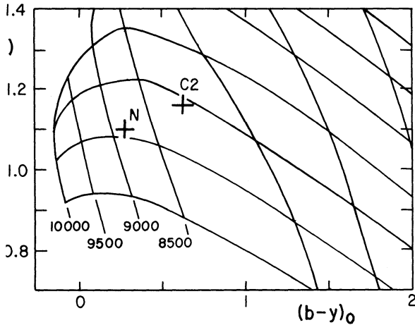
Fig. 5. Position of the stars in the theoretical grids of Relyea & Kurucz (1978).
