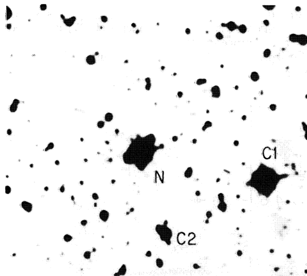
Fig. 3. Enlargement of an INAOE Schmidt plate of the non-stellar appearance of the proposed newly determined reflection nebula. The stars C1 and C2 have been taken as references.
