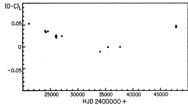
Fig. 8a. O-C residuals versus HJD for RZ Tau using the linear ephemeris HJD_{min} = 2437676.575 + 0.4156731 E .
