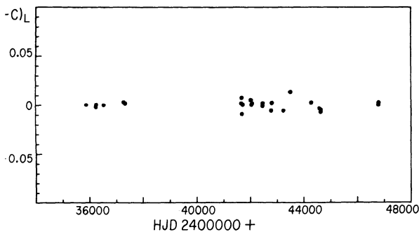
Fig. 6d. O-C residuals versus HJD for ER Ori for the last group of minima using the linear ephemeris HJD_{min} = 136508.7851 + 0.4233994 E .
