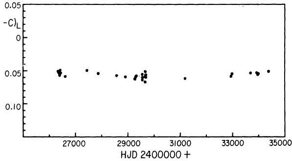
Fig. 6b. O-C residuals versus HJD for the first group of minima using the linear ephemeris HJD_{min} = 136508.7851 + 0.4233957 E .
