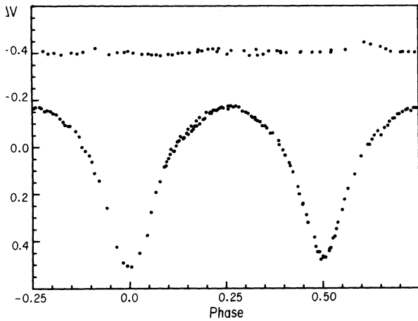
Fig. 4a. Light curves in phase for the observed nights at JAB-SPM in the V filter of YY Eri. The period used was P = 0.3214959 d, found in the present paper. The points in the upper part correspond to C1-C2.
