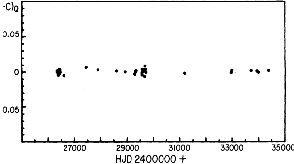
Fig. 6c. O-C residuals versus HJD for the first group of minima using the quadratic ephemeris HJD_{min} = 136508.7851 + 0.4233979 E + (1.51 \times 10^{-10}) E^2/2 .
