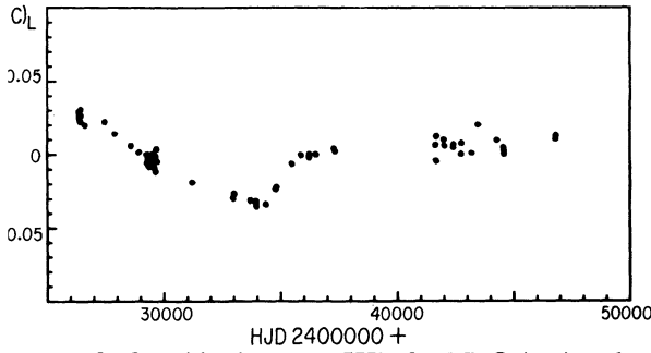
Fig. 6a. O-C residuals versus HJD for ER Ori using the linear ephemeris for the complete set of minima HJD_{min} = 2436508.7851 + 0.4233990 E .
