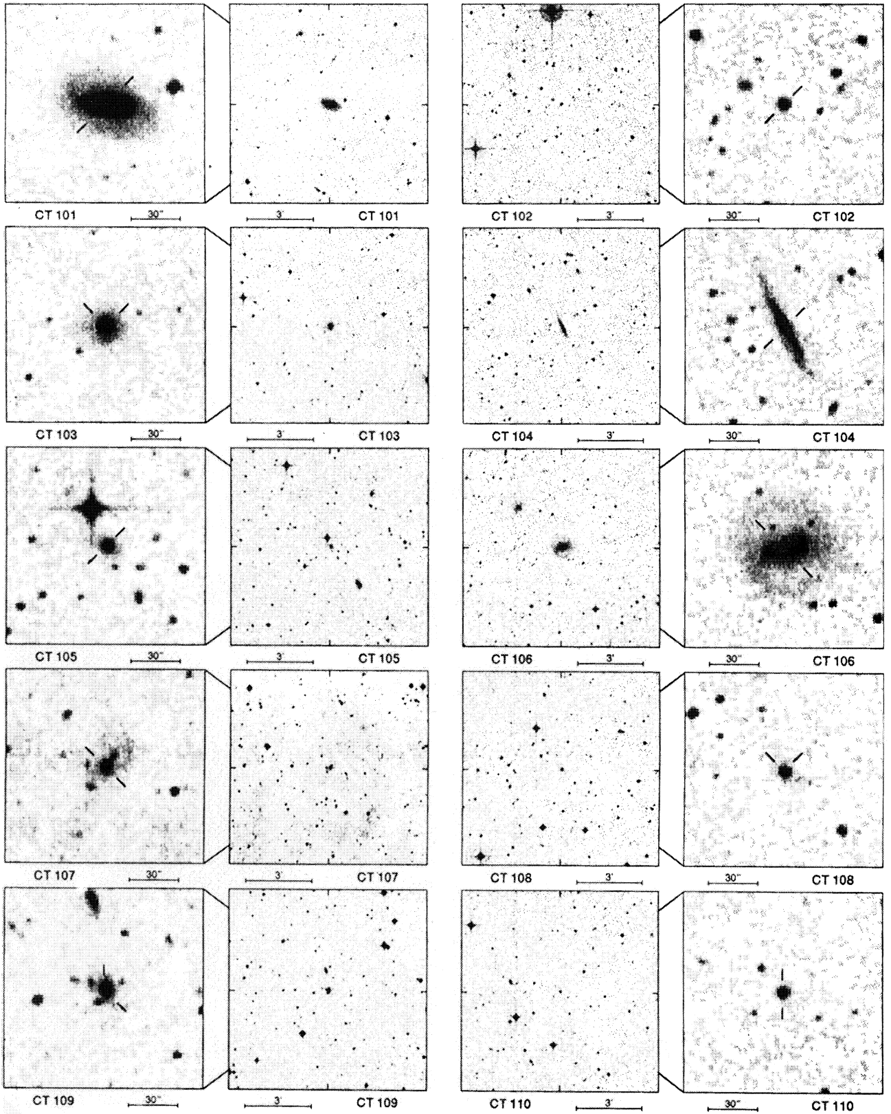
Fig. 1d. Finding charts from the (DSS).
