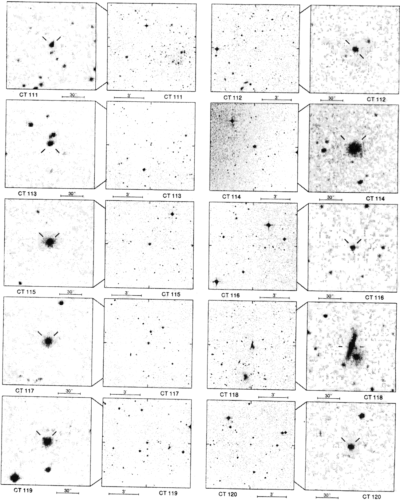
Fig. 1e. Finding charts from the (DSS).
