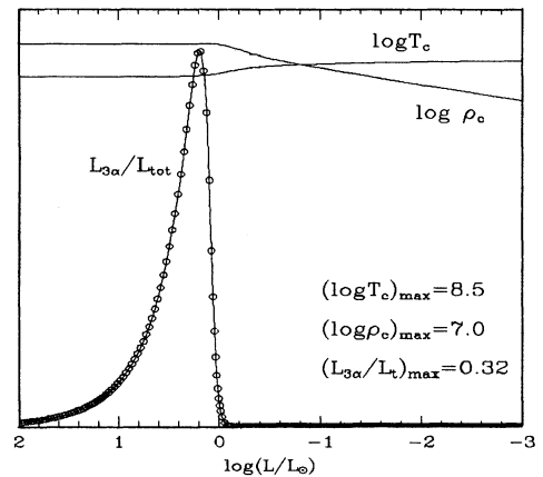
Fig. 2. Internal evolution of the \eta = 1.0 model. The variables are normalized to the values indicated.
