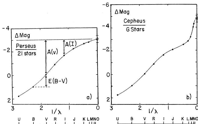
Fig. 3. Interstellar reddening laws for Perseus and Cepheus, after Johnson (1968). The asymptote approached by the Perseus curve, and arrows defining A_V , A_I , and E(B-V) , have been added. The long-wavelength data for Cepheus depends almost entirely upon a single star, \mu Cep, an M2 Ia supergiant with a substantial circumstellar dust shell.
