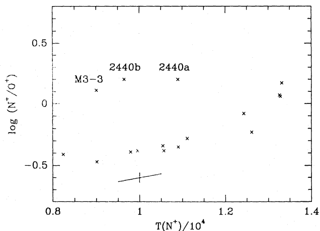
Fig. 5. \text{N}^{+}/\text{O}^{+} vs. T(\text{N}^{+}) . A typical error is presented, where the dependence of \text{N}^{+}/\text{O}^{+} on temperature is considered. The vertical bar corresponds to an error in the I(6583)/I(3727) ratio of 0.04 dex.
