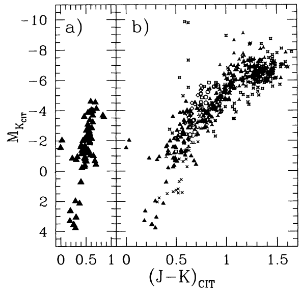
Fig. 3. a) Colour-magnitude ( M_{K_{CIT}} versus (J-K)_{CIT} ) diagram for the halo stars studied in this paper. b) The same colour-magnitude diagram in which the halo stars are seen in comparison with stars from other stellar populations. The symbols are as for Figure 1b. Note how the halo stars extend to bluer colours and fainter magnitudes.
