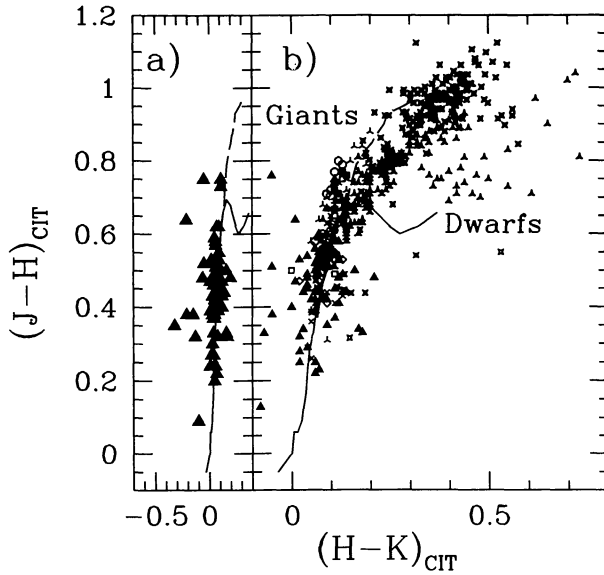
Fig. 1. a) JHK diagram for the halo stars studied in this paper. The intrinsic dwarf (solid line) and giant (broken line) sequences from Bessell & Brett (1988) are shown. b) JHK diagram for the halo stars in this paper and stars belonging to other stellar populations: M3 (open circles), M13 (open squares), M92 (open diamonds), M67 (crosses), 47 Tucanae (skeletal triangles), BW stars from Frogel & Whitford (1987) (three pointed stars) and BW stars from Ruelas-Mayorga & Teague (1992a) (four pointed stars).
