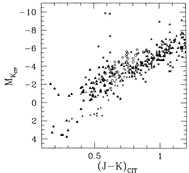
Fig. 4. The same colour-magnitude diagram for a more restricted section of the plot.
