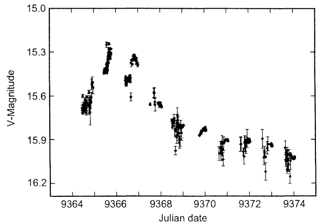
Fig. 2. Details of the flare behaviour in V-band.
