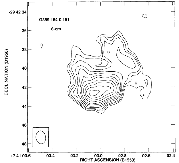
Fig. 4. VLA radio continuum map at 6 cm (A+B configurations) toward G359.164-0.161. Contour levels are -4, -3, 3, 4, 5, 7, 9, 12, 15, 20, 25, 30, 35 , and 40 times 31 \mu\text{Jy beam}^{-1} .
