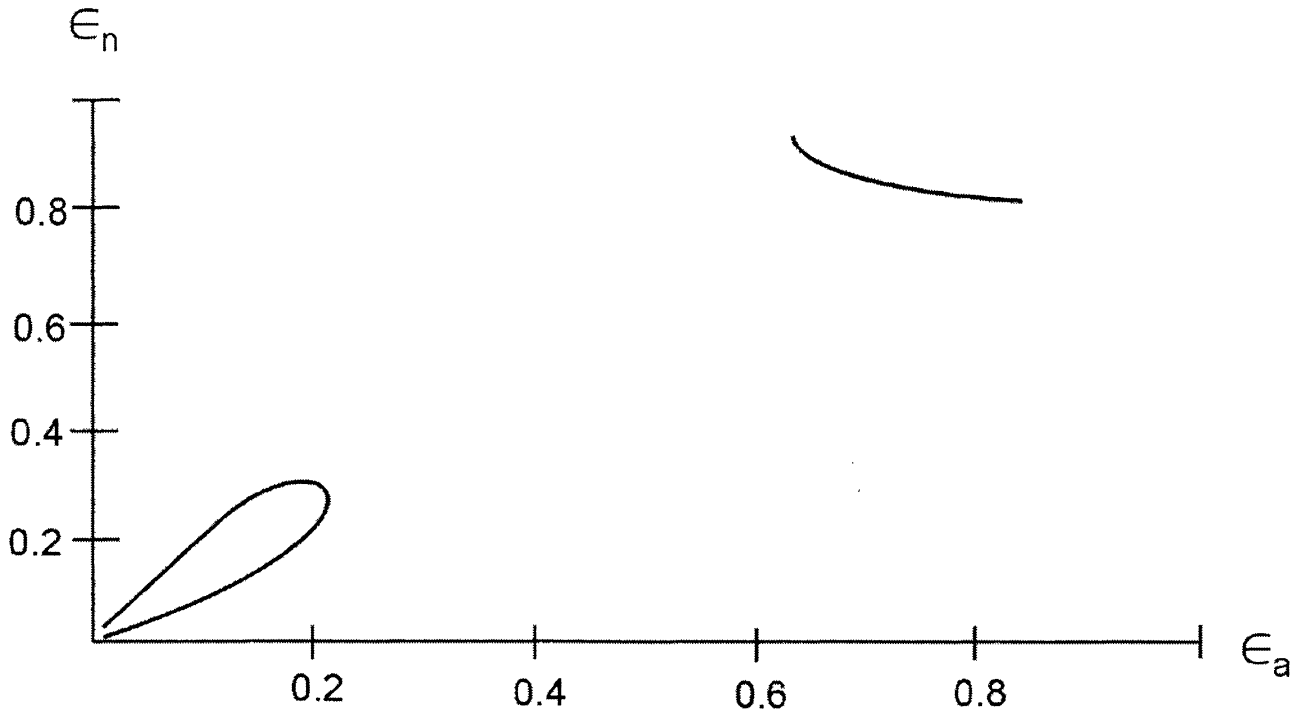
Fig. 3. The behavior of \epsilon_n as a function of \epsilon_a of the bifurcation points for \varepsilon = 5 , according to Table 2.
