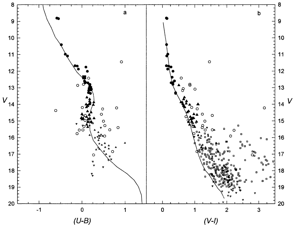
Fig. 4. a. The V versus (U-B) diagram. The solid line represents the ZAMS (Schmidt-Kaler 1982); symbols have the same meaning as in Fig. 3 a . b. The V versus (V-I) diagram. The solid line shows the relation for main sequence stars from Cousins (1978); symbols as in Figure 3 a .
