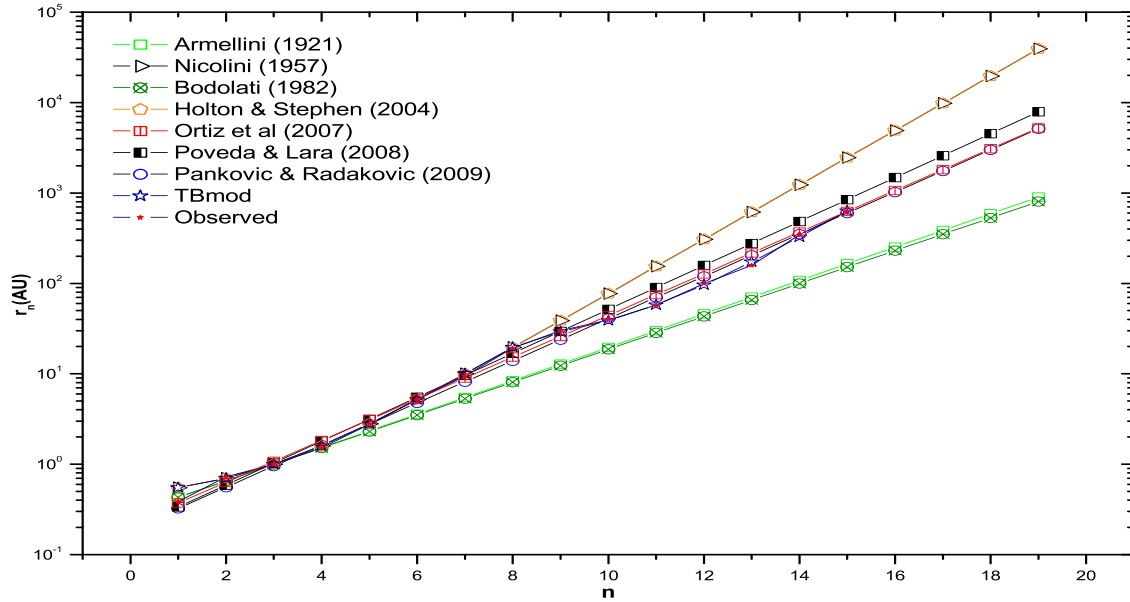
Fig. 2. Titius-Bode models of several authors including the TBmod variant proposed in this work. It is to be noted that the models are distributed above or below the real TB distribution of planets and the TBmod curvilinear path, which coincides with the values of the observed semi-major axes. We have chosen the logarithmic scale to better visualize the linear trace of the other six models. The color figure can be viewed online.
