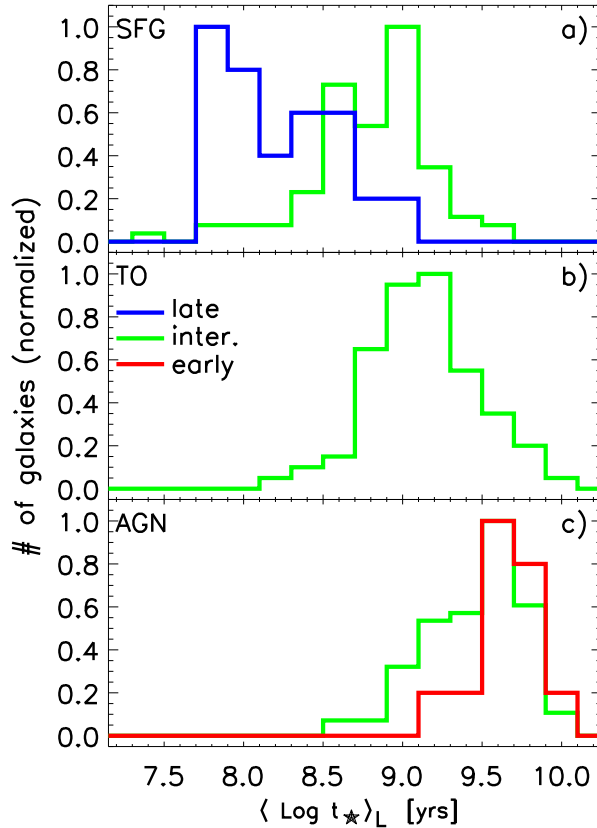
Fig. 12. Distributions of mean ages of stellar populations for galaxies with different activity types and different morphologies.
