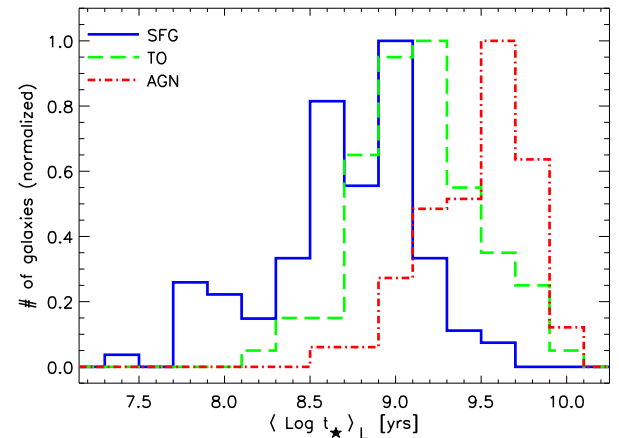
Fig. 11. Distributions of mean ages of stellar populations for galaxies with different activity types.
