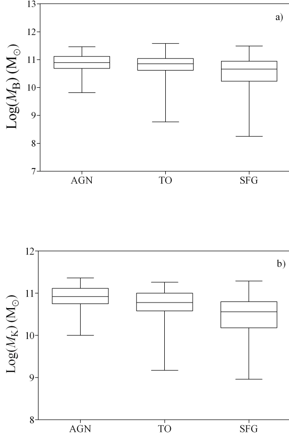
Fig. 9. Box-whisker plots for the total masses in galaxies showing different activity types; (a) M_B and (b) M_K .
