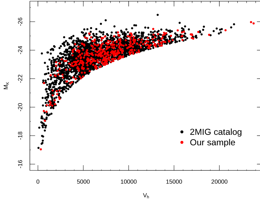
Fig. 4. Comparison of absolute K magnitude vs. heliocentric velocity for the 2MIG catalog and our subsample of 292 isolated NELGs.
