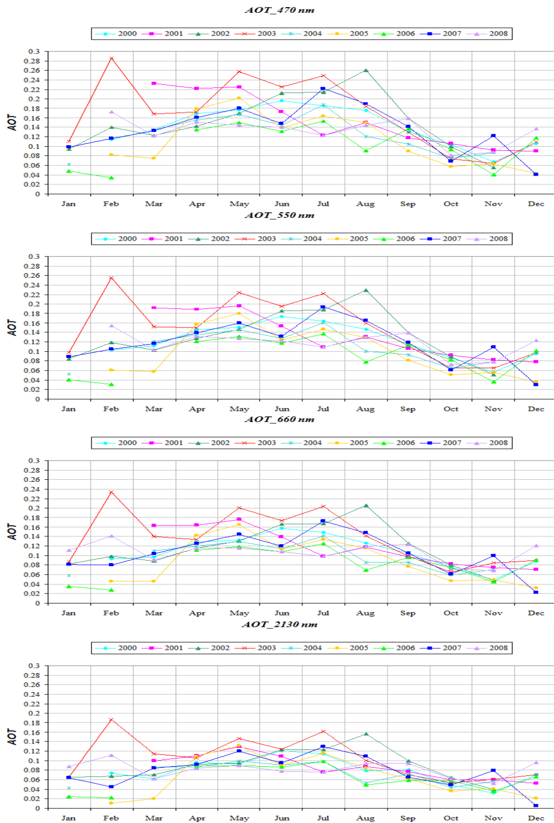
Fig. 4. Annual AOT behavior at the SPM location by monthly average at 470 nm (top), 550 nm (second from top to bottom), 660 nm (third from top to bottom), and 2130 nm (bottom).
