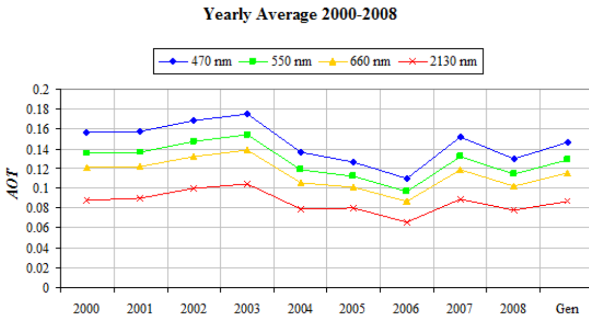
Fig. 5. Annual aerosol optical depth average at SPM at 470, 550, 660 and 2130 nm during the years 2000–2008.
