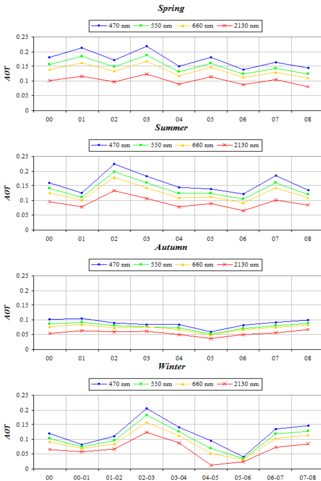
Fig. 1. The average seasonal (March to May for spring, June to August for summer, September to November for autumn, and December to February for winter) AOT above SPM over the years 2000–2008.
