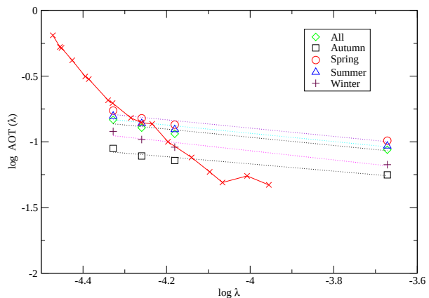
Fig. 7. Wavelength dependence of average atmospheric extinction ( \kappa_\lambda ) from Schuster & Parrao (2001) represented with \times symbols, compared to the aerosol optical depth spectral values obtained from MODIS data for the San Pedro Mártir observatory site.
