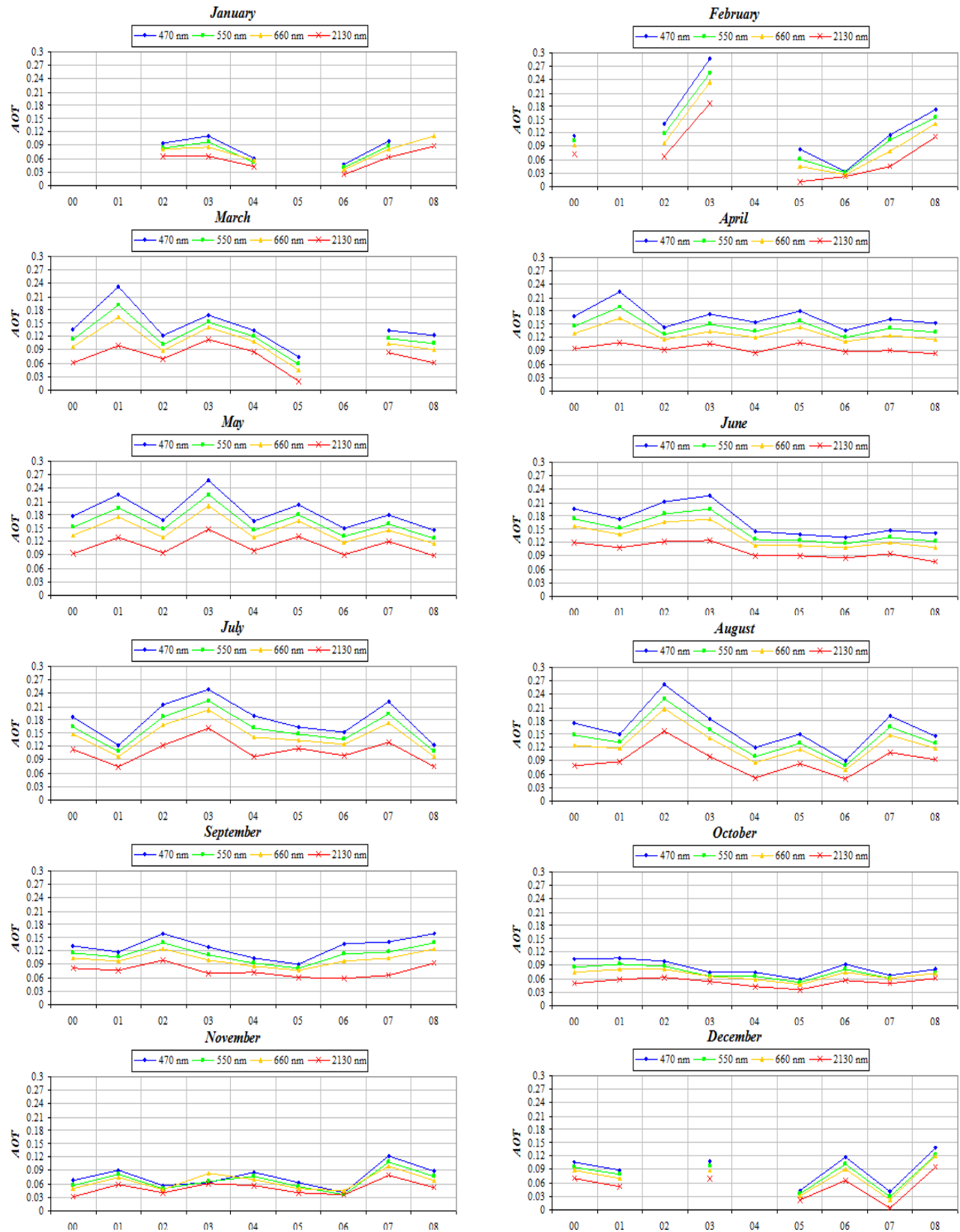
Fig. 3. Monthly Average (January to December) 2000–2008.
