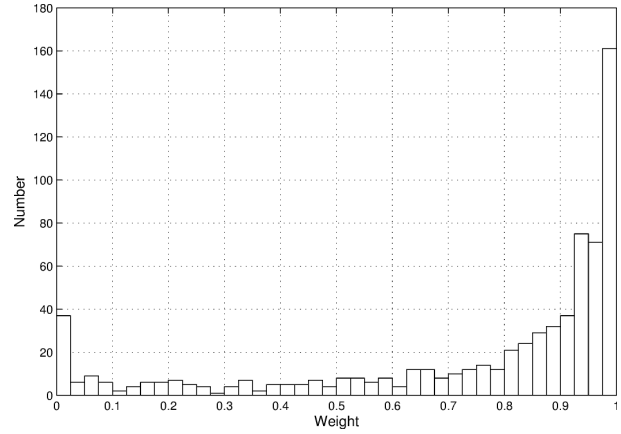
Fig. 2. Histogram of Welsch weights.
