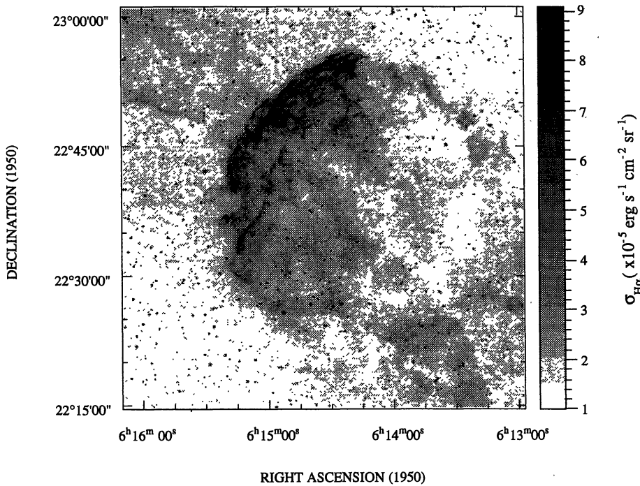
Fig. 1. Flux calibrated CCD image of IC 443 in H \alpha .
