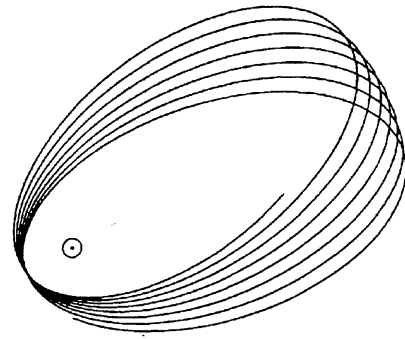
Fig. 2. Moving Keplerian ellipse.
