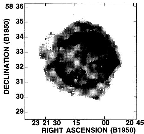
Fig. 1. Example of shell-type SNR: Cassiopea A (Courtesy of NRAO).
