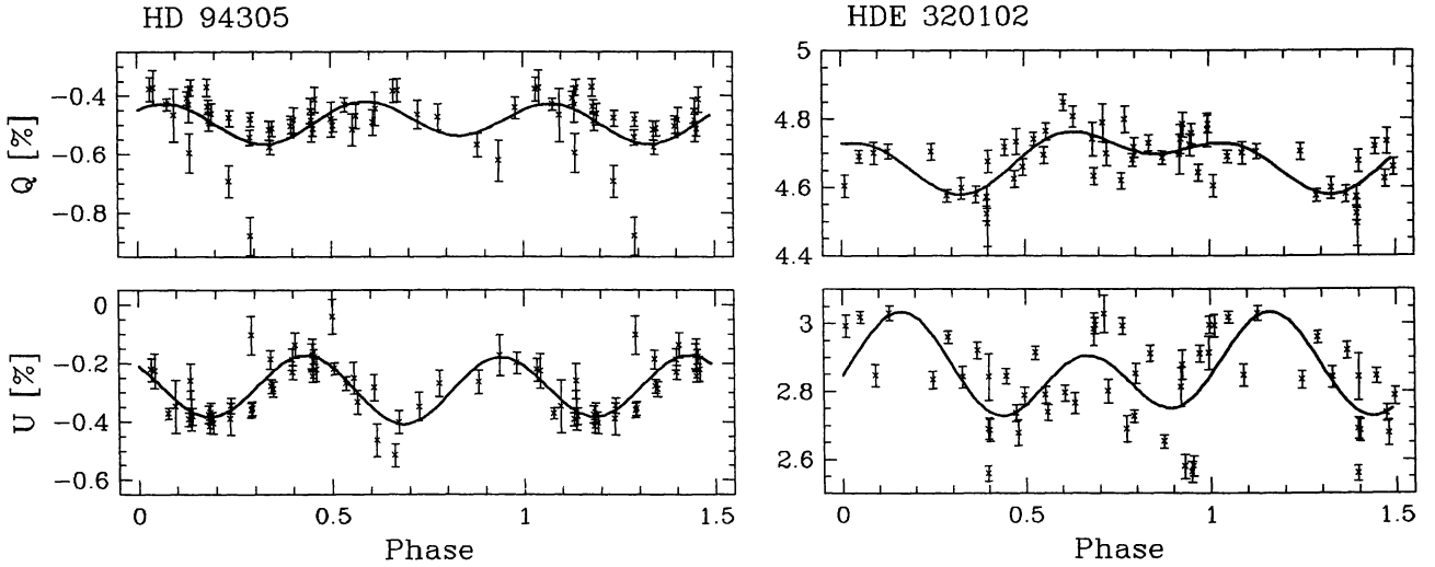
Fig. 2. The variation of the Stokes parameters, Q and U , plotted vs. orbital phase of the binaries. The solid lines are the best fit to a Fourier series up to second-harmonic terms.
