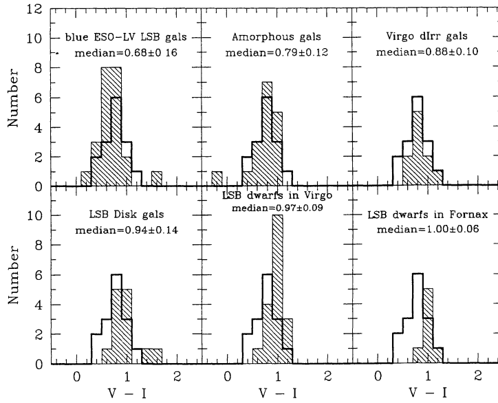
Fig. 1. Comparison of the colours of the extensions of H II galaxies (solid line histograms) control samples of dwarf galaxies (hatched histograms): Blue ESO-LV LSB galaxies (Rönnback & Bergvall 1994); Amorphous galaxies (Gallagher & Hunther 1987); Virgo dIrr galaxies (Bothun et al. 1996); LSB disk galaxies (McGaugh & Bothun 1994); LSB dwarf ellipticals in Virgo (Impey et al. 1988); LSB dwarf ellipticals in Fornax (Bothun et al. 1991). For H II galaxy these values are V - I = 0.74 \pm 0.14 and R - I = 0.51 \pm 0.18 .
