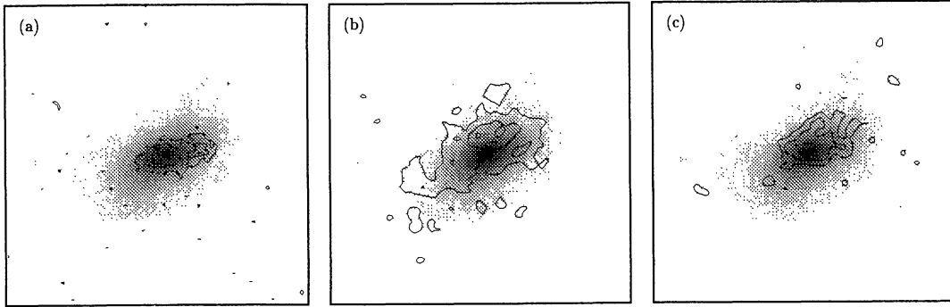
Fig. 3. He 2-10. Greyscale: 2\ \mu\text{m} continuum (the faint isophotes have been enhanced to highlight the eastern star-forming region). Contours: (a) \text{Br}\gamma , (b) 1-0\ \text{S}(1) , (c) \text{He I} . The spatial resolution of the line images degrades from (a) to (c). The figures are 20 arcsec (900 pc) across; north is up and east is left.
