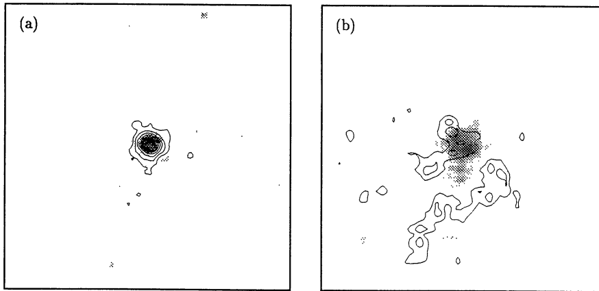
Fig. 1. II Zw 40. Greyscale: 2\ \mu\text{m} continuum (the difference between (a) and (b) is due to variations in spatial resolution); Contours: (a) \text{Br}\gamma , (b) 1-0\ \text{S}(1) . The figures are 30 arcsec (1.5 kpc) across; north is up and east is left.
