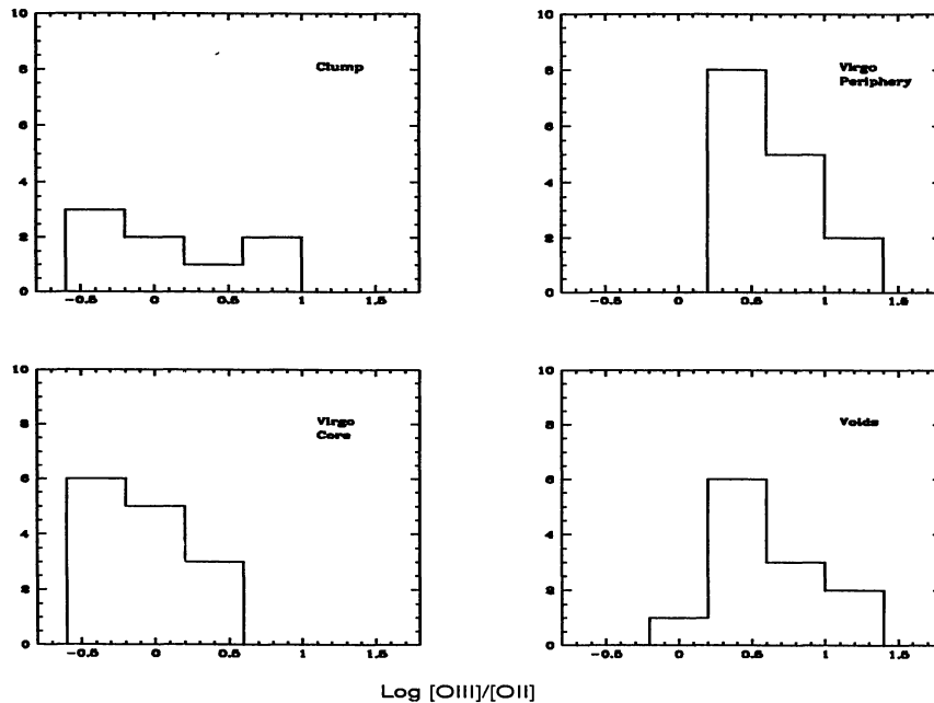
Fig. 1. The behaviour of the excitation, measured by the [\text{O III}]/[\text{O II}] ratio, for a sample of star-forming dwarf galaxies located in environments with different density, including low density objects from nearby voids and in the periphery of the Virgo cluster/Local Super-cluster, and high density objects located in the Virgo cluster and in a dense group/clump of galaxies. The higher excitation objects of the sample are found in the lower density environments.
