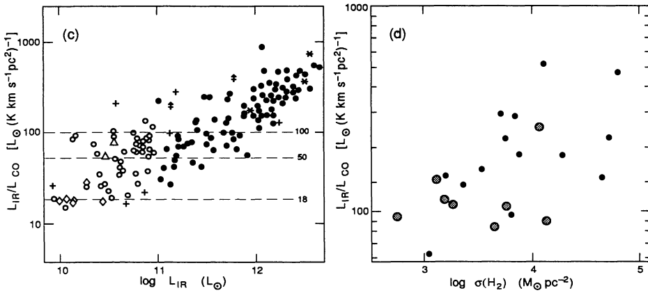
Fig. 2. (a) L_{\text{IR}}/L'_{\text{CO}} vs L_{\text{IR}} . The dashed lines represent mean values for nearby ‘normal’ spirals ( L_{\text{IR}}/L'_{\text{CO}} \sim 18 ), nearby starburst galaxies ( L_{\text{IR}}/L'_{\text{CO}} \sim 50 ), and the most extreme star-forming GMC cores in the Milky Way ( L_{\text{IR}}/L'_{\text{CO}} \sim 100 ). Solid and open circles represent LIGs and lower luminosity BGS galaxies, respectively (see Sanders et al. 1991; Solomon et al. 1996). Open triangles refer specifically to the nearby starburst galaxies M82 and NGC 253, and open diamonds represent the Milky Way and 5 similar nearby spiral galaxies (see Sanders et al. 1991). Asterisks refer to optically selected QSOs that have been detected in CO: I Zw1 (Barvainis et al. 1989), Mrk 1014 (Sanders et al. 1988), 3C 48 (Scoville et al. 1993). The ‘+’ signs represent powerful radio galaxies detected by IRAS (see Mazzarella et al. 1993; Evans 1996). (b) Correlation of the central concentration of molecular gas with the L_{\text{IR}}/L'_{\text{CO}} ratio for LIGs in the IRAS BGS (Scoville et al. 1991; Bryant 1996). Small black and larger gray circles represent objects where the spatial resolution was sufficient to resolve circumnuclear regions of <1 kpc and 1–2 kpc diameter respectively.
