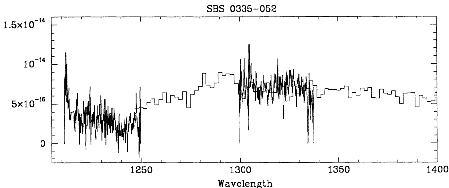
Fig. 3. HST -GHRS spectra of SBS 03350052 for the \text{Ly}\alpha and the O I regions superimposed to the IUE SWP spectrum.
