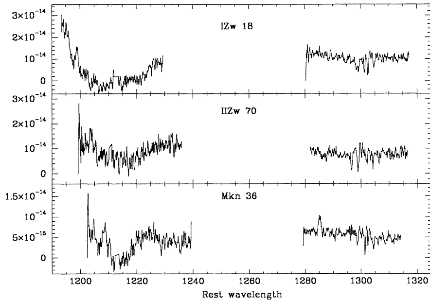
Fig. 2. HST -GHRS spectra for 3 galaxies with no \text{Ly}\alpha emission. In this case the \text{Ly}\alpha region shows a broad damped absorption. Both the \text{Ly}\alpha and the O I regions are displayed.
