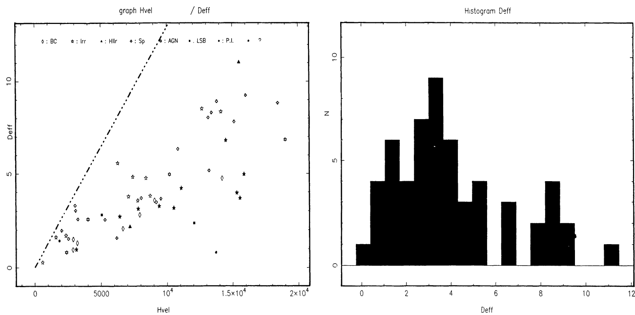
Fig. 2. a) effective diameter (kpc) vs. velocity ( \text{km s}^{-1} ) (dashed-dotted line: limiting effective diameter D = 10'' ). b) Effective diameter distribution (kpc).
