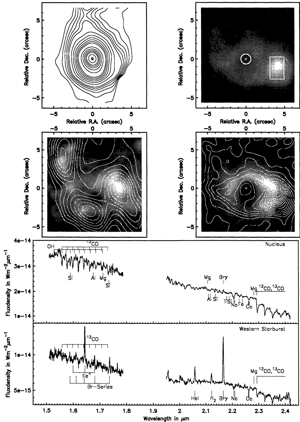
Fig. 1. Top left: contour plot of the continuum flux at 1.65 \mu\text{m} . Top right: Line map of Br \gamma at 2.166 \mu\text{m} . Middle left: Line map of H 2 1-0 S(1) at 2.12 \mu\text{m} (grayscale) vs. HCN-emission (contours) from Downes et al. (1992). Middle right: Line map of [Fe II] at 1.644 \mu\text{m} (grayscale) vs. Br \gamma emission from Fig. 1a) (contours). Resolution of all maps is \approx 1'' . Bottom: H and K spectra of the central 1.25'' (12 pc) and the western starburst region.
