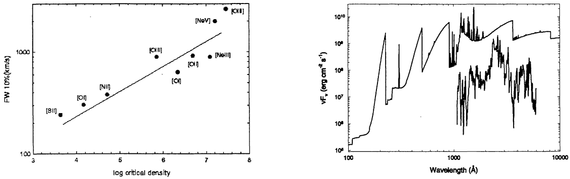
Fig. 4. a) Line width-critical density correlation for the NLR LOC calculations. Points indicate predicted widths for individual lines, and the line is a fit to the points. b) Emission from a BLR cloud. The upper curve is the total emission and the lower is the Fe II emission alone.
