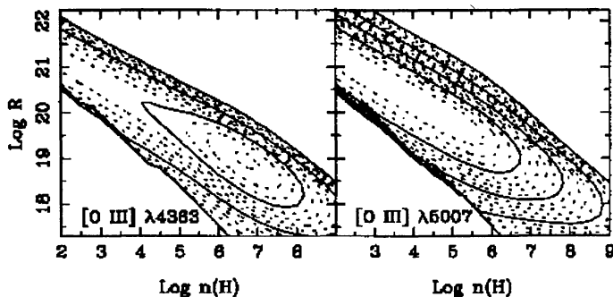
Fig. 3. Predicted [O III] 4363 and 5007 equivalent width as a function of the cloud density and the distance from the AGN nucleus. Heavy lines are 1 dex increases in equivalent width, starting at 1.
