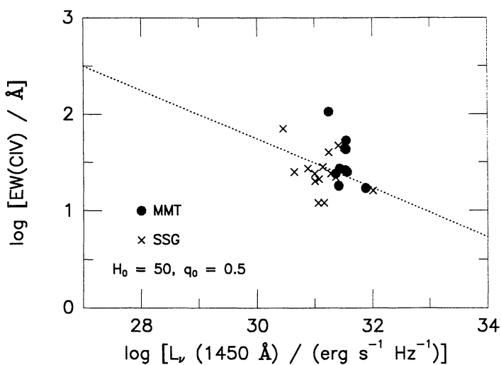
Fig. 2. Rest-frame EW(C\text{ IV}) as a function of rest-frame 1450 Å luminosity for z > 4 QSOs. Filled circles represent MMT measurements with continuum photometry from Storrie-Lombardi et al. (1996); crosses are measurements published by Schneider et al. (1991). The dotted line represents the empirical trend found by Osmer et al. (1994) for QSOs at Z = 2 - 3 .
