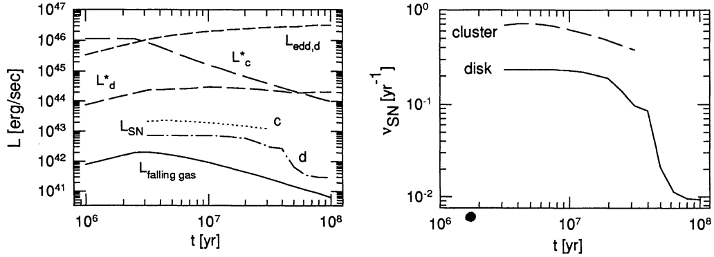
Fig. 1. a ) Evolution of a stellar cluster and its disk core, with ( M_l = 1 M_\odot , M_u = 120 M_\odot ); N_c = 3 \times 10^8 ; R_c = 53 pc; total cluster mass M_c = 9.5 \times 10^8 M_\odot ; R_d = 2.6 pc; total number of stars in the disk N_d = 9 \times 10^7 ; stellar mass in the disk M_d = 1.6 \times 10^8 M_\odot ; and gas density in the disk \rho_d = 9 \times 10^7 g cm ^{-3} . Luminosity sources shown: L_{SN} - total SN luminosity in the cluster and disk; L_{falling-gas} - rate of energy released by the infalling gas in the disk; L^* - starlight in the cluster and disk; and L_{edd,d} - the Eddington luminosity limit in the disk. For a cluster with a mass ten times larger (smaller), all the luminosity values increase (decrease) by an order of magnitude; b ) Rates of supernovae production, \nu_{SN} , in the cluster and the disk.
