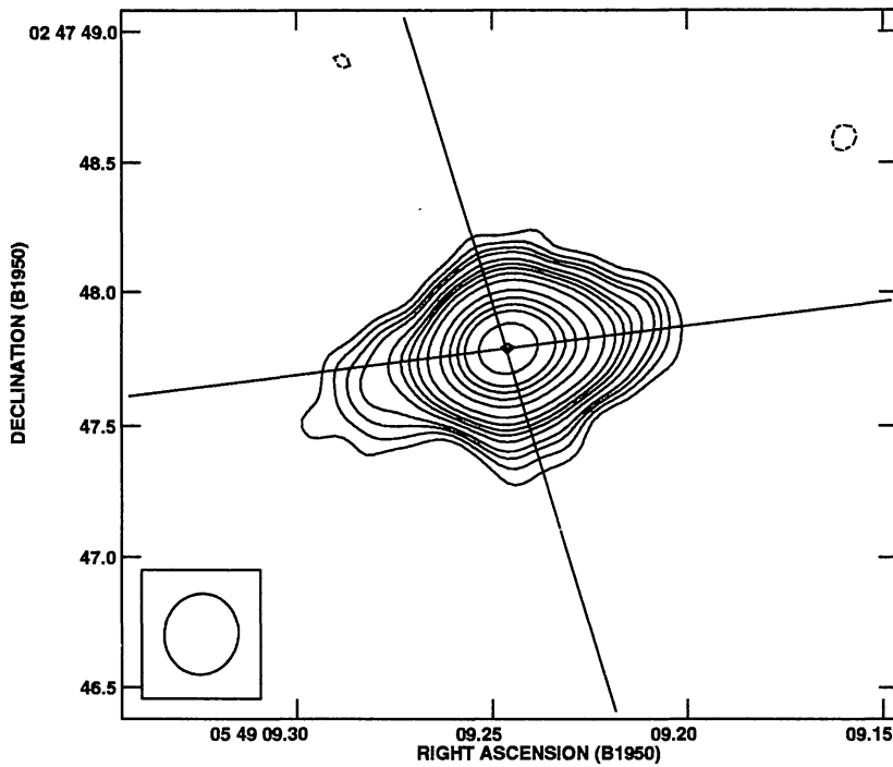
Fig. 3. VLA map at 3.6 cm wavelength of the exciting source at the core of the quadrupolar outflow in HH 111. Contours are -3, 3, 4, 5, 6, 8, 10, 12, 15, 20, 30, 40, 50, 60, 80 , and 100 times the rms noise of 5.4 \mu\text{Jy beam}^{-1} . The half power contour of the synthesized beam is also shown. The straight lines give the position angles of the two flows in the region.
