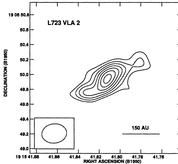
Fig. 2. VLA map at 3.6 cm wavelength of the source VLA 2 at the core of the quadrupolar outflow in L723. Contours are -3, 3, 4, 5, 6, 7, 8 , and 9 times the rms noise of 11 \mu\text{Jy beam}^{-1} . The half power contour of the synthesized beam is also shown. The major axis of VLA 2 aligns with the axis of the large CO lobe pair that has a position angle \text{PA} \simeq 110^\circ .
