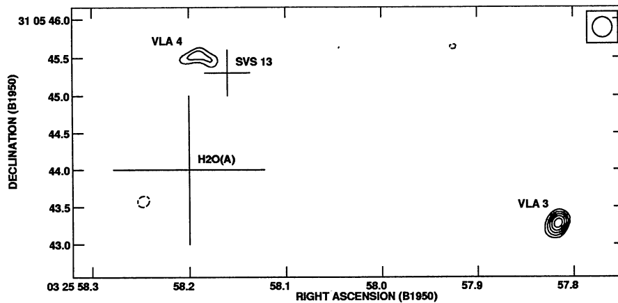
Fig. 1. Natural-weight VLA map at 3.6 cm wavelength made in the A configuration of the sources VLA 3 and VLA 4 at the central region of the HH 7–11 outflow. The positions of the near-infrared/optical source SVS 13 and of the water maser H 2 O(A) are indicated with crosses. The source VLA 4 is associated with the infrared/optical source SVS 13. The source VLA 3 is a newly detected object that has been proposed by Rodríguez et al. (1997) as a candidate to excite the HH 7–11 outflow. The half power contour of the beam is shown in the top right corner. Contour levels are -3, 3, 4, 5, 6 , and 7 times the rms noise of 20 \mu\text{Jy beam}^{-1} .
