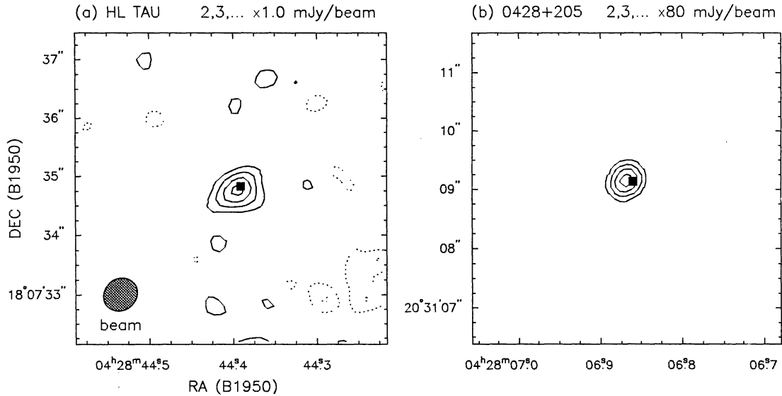
Fig. 4. (a) VLA map at 7-mm of HL Tau. At this relatively low angular resolution ( 0''.5 ) the emission from the dust disk is detected. (b) VLA map at 7-mm of the point source 0428+205. The half power contour of the synthesized beam for the HL Tau map is shown.
