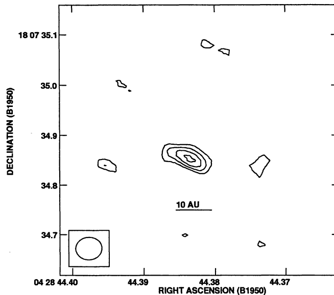
Fig. 5. VLA map at 7 mm wavelength of HL Tau. At the high angular resolution ( 0''.04 ) of this map only the compact thermal jet is detected. Contours are -4 , -3 , 3 , 4 , 5 , and 6 times 0.17 \text{ mJy beam}^{-1} . The half power contour of the beam is shown, as well as a scale of 10 AU (assuming a distance of 140 pc).
