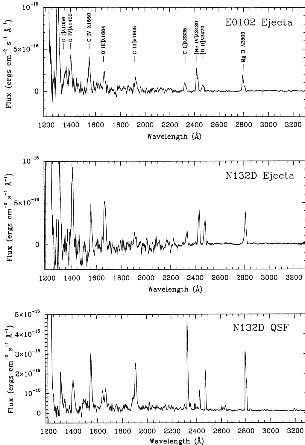
Fig. 3. UV spectra of N132D and E0102.2–7219 obtained with the FOS aboard HST . The aperture positions are marked in Figs. 1 and 2. For N132D, the two O-rich positions were shifted to a common velocity and co-added to increase the S/N. Major emission lines in the O-rich ejecta are labeled in the top panel. The spectra of the ejecta in E0102 and N132D are similar, but the QSF spectrum shows He II λ1640 and Si III] λ1885 emission, plus a number of lines near 2600 Å, that are not present in the ejecta. The E0102 spectrum was corrected for extinction using E(B - V) = 0.1 , and the N132D spectra were corrected using E(B - V) = 0.2 .
