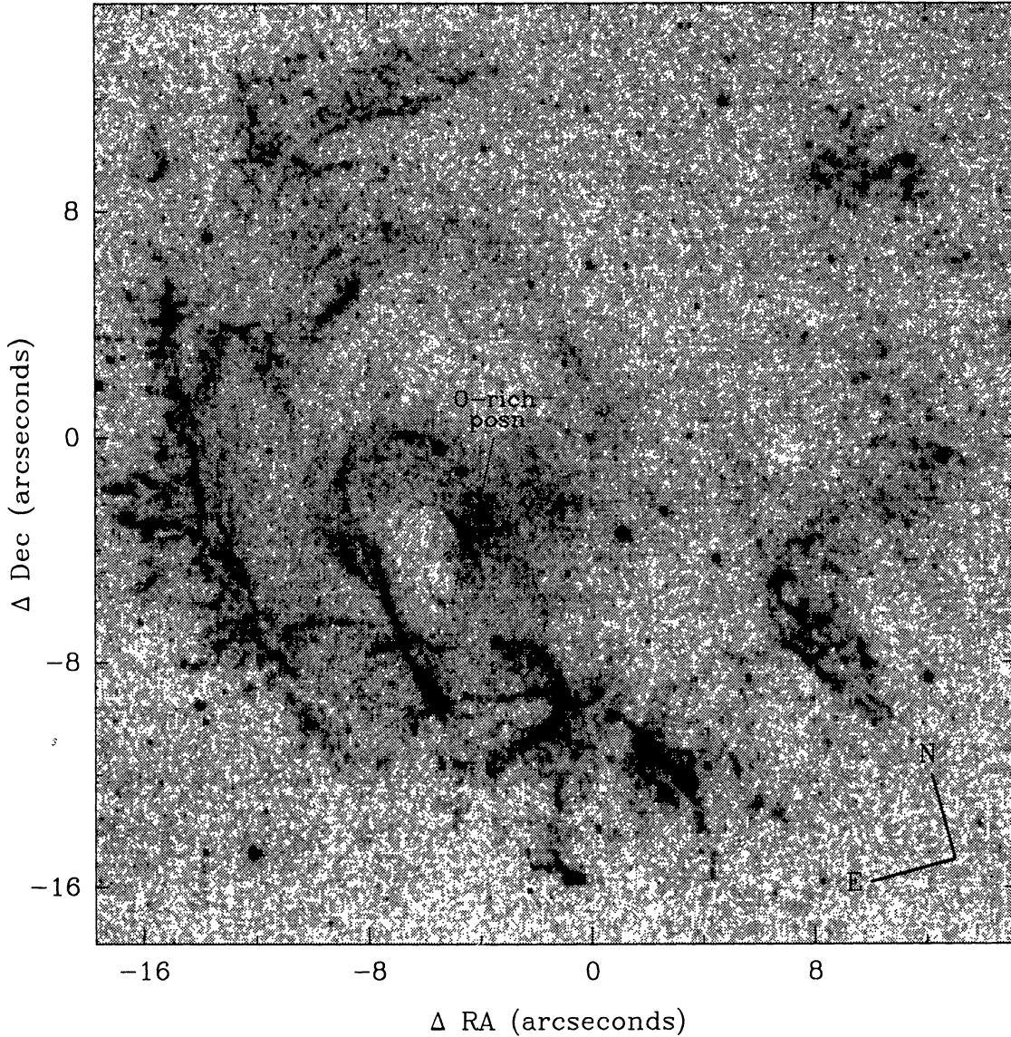
Fig. 2. WFPC2 image of E0102.2-7219 in [\text{O III}]\lambda 5007 . The position of the FOS aperture in the O-rich debris is marked. Due to the large velocity range in the ejecta, a substantial number of filaments in the center of the remnant are excluded from the filter bandpass. Overall, however, the morphology of this remnant bears a striking resemblance to Cas A. The position (0,0) is at coordinates 1:04:01.4, -72:01:54 (2000), and the orientation is indicated in the lower right corner.
