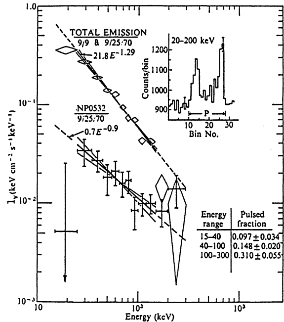
Fig. 6. A later measurement by UCSD separated the hard X-ray spectrum of the pulsed component from the nebula component, and showed the pulsed component has a flatter power-law spectrum in this energy range.
