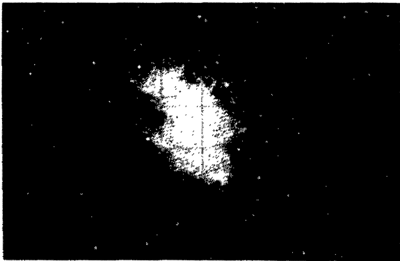
Fig. 1. Black and white version of a color photo of the Crab Nebula. The size is several arc minutes. The red emission from the filaments in the outer regions is due primarily to the excited states of N and O, while the blue continuum in the center is due to synchrotron radiation in an \sim 10^{-4} gauss field. The blue south star to the left of the central region is the pulsar.
