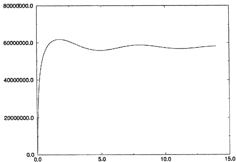
Fig. 4. Lorentz factor vs. phase for pickup from 10^6 radii. Notice that although the field weakens markedly, the electron remains coupled to some degree.
