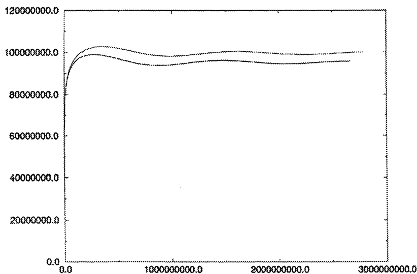
Fig. 5. Lorentz factor vs. distance in wave zone radii for resonant (upper) and non-resonant particles (lower).
