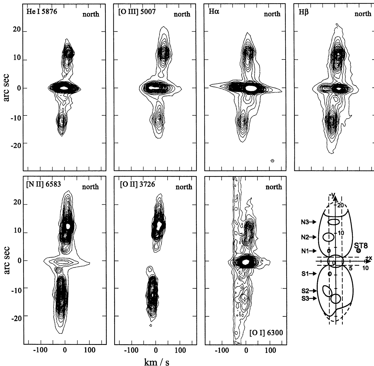
Fig. 1. Isocontours of bright emission lines ( H\alpha , H\beta , [O III], He I, [O II], and [N II]). The contours show moderate velocity in the lobes and high velocities in the nucleus. In H\alpha and H\beta the significant larger reddening at the nucleus can be noticed. In H\alpha , H\beta , and [O III] the central emissions have two maxima. The peak in H\alpha is redshifted , while that in [O III] is blueshifted from the mean velocity of the object. The He I emission is wide and shows a single peak in the nucleus at the systemic velocity of M2-9. A bright low ionization knot displaced ( \sim -20 \text{ km s}^{-1} ) 3'' South from the nucleus is observed in [O II] and [N II]. Also included is a diagram of the nebula and condensations from Kohoutek & Surdej (1980) with the slit indicated.
