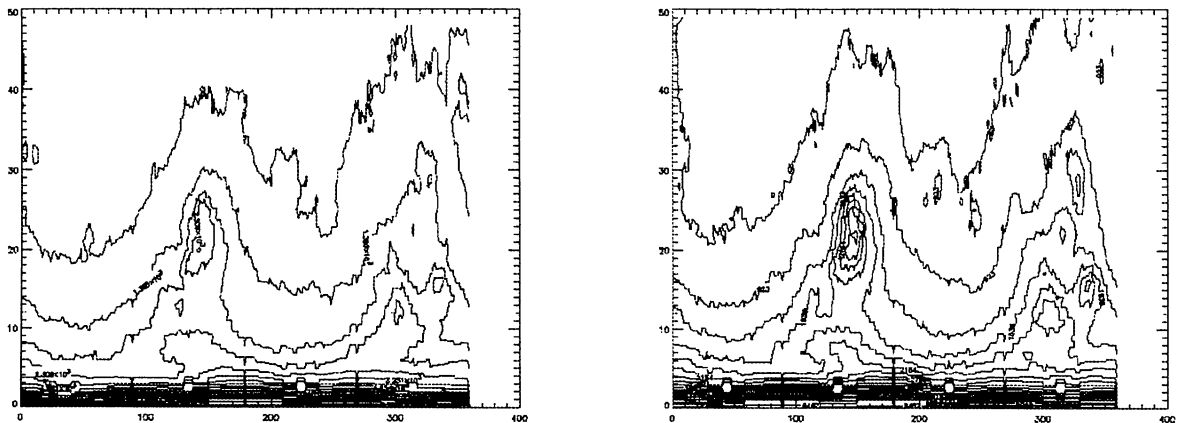
Fig. 3. Structure of irregular galaxy NGC 4449 in the R band (left) and in the J band (right). We are searching structures in this galaxy, analysis in other bands probably say us if exist them.
