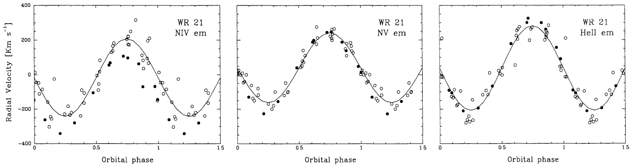
Fig. 1. Radial velocity variations of NIV 4058 Å (left), NV 4603 Å (center) and HeII 4686 Å (right) emissions in the spectrum of WR 21, phased with the improved period. Filled circles represent our new CASLEO data, open circles previous observation (cf. Table 1). Continuous lines represent the orbital solutions from Table 1.
