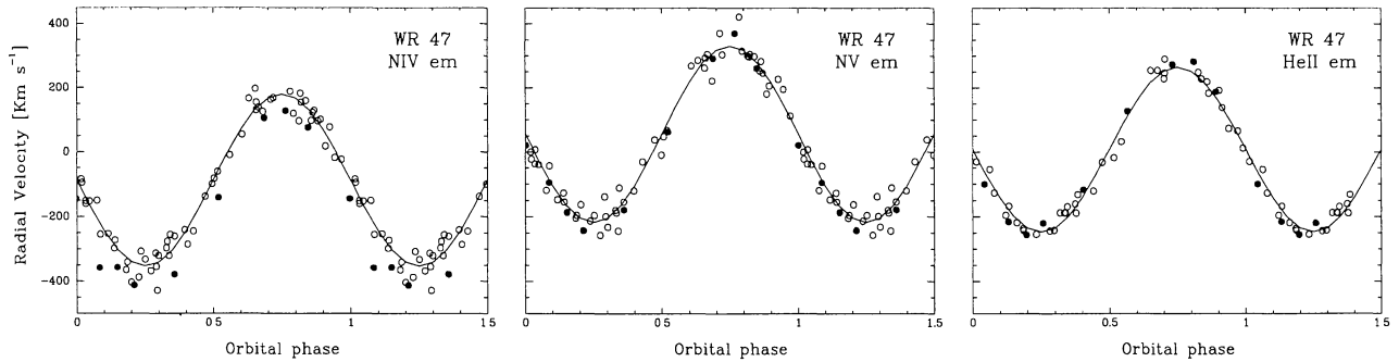
Fig. 3. Idem Fig. 1, but for WR 47.
