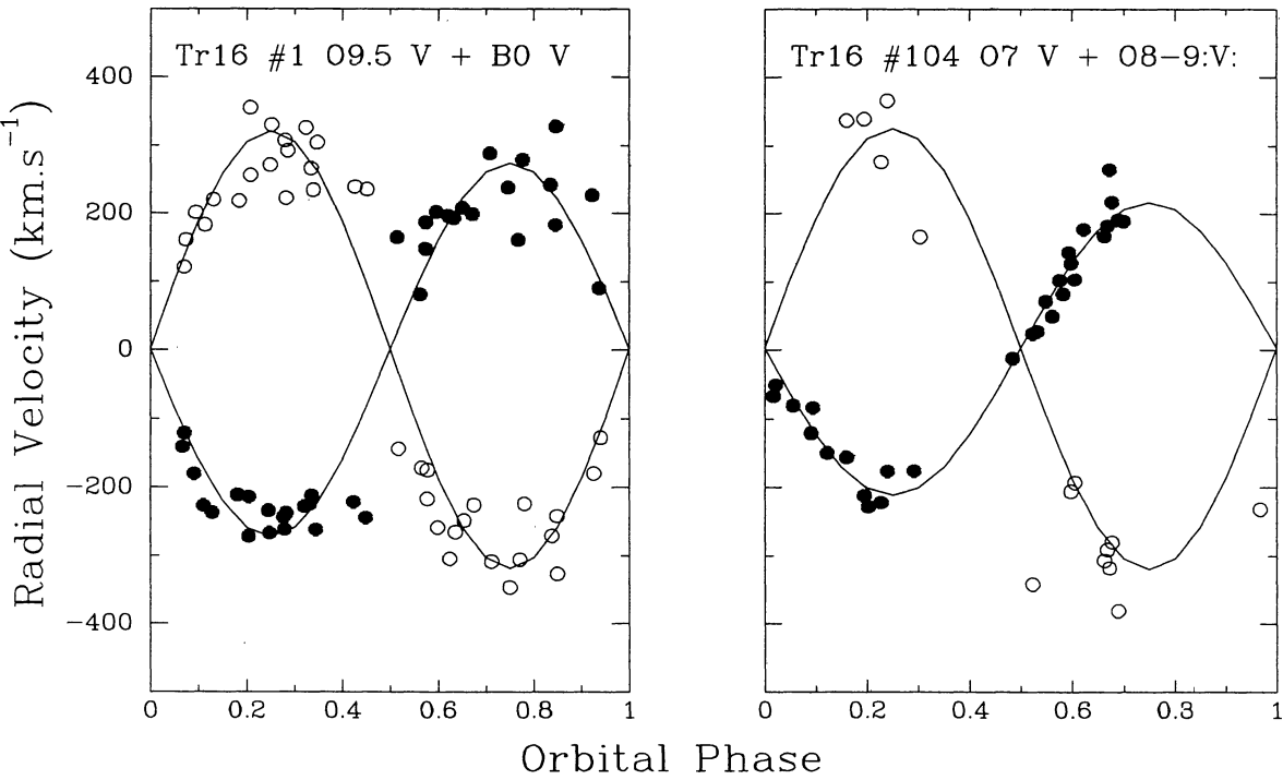
Fig. 1. Radial velocity orbits of Tr 16 #1 and Tr 16 #104.
