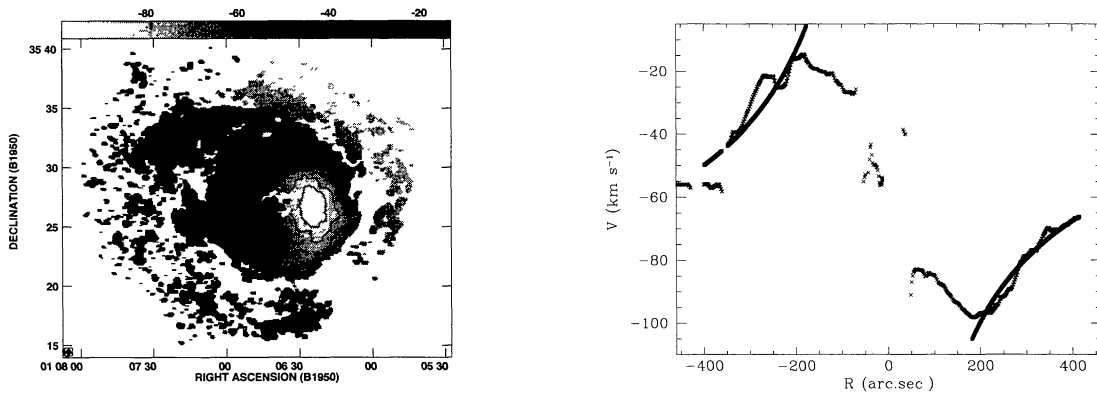
Fig. 1. Left : grey scale flux range = -99.6 – -14.6 \text{km s}^{-1} , contour levels are drawn at -90 , -80 , -70 , -60 , -50 , -40 , -30 and -20 \text{km s}^{-1} . Right : observed rotation curve, uncorrected for inclination; crosses: observations; solid squares: Keplerian.
