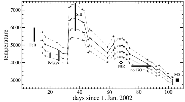
Fig. 1. The evolution of the photosphere temperature using blackbody fits to the photometry at different interstellar foreground extinction (from top to bottom: E(B-V) = 0.8, 0.7, 0.6 , and 0.5 ). From the spectroscopy (Fe II at day 10 and Si II only just after the February outburst) we derive 0.7 < E(B-V) < 0.9 . Zwitter & Munari (2002) find K-type just before the outburst. This leads to somewhat lower values. The NIR continuum (Geballe et al. 2002) suggests values below 0.5 . The absence of TiO bands during March limits E(B-V) to values above 0.7 mag. Finally, the spectroscopy of Rauch & Kerber (2002) give us 0.7 < E(B-V) < 0.8 . The value of E(B-V) = 0.7 is the best fit to the whole time series.
