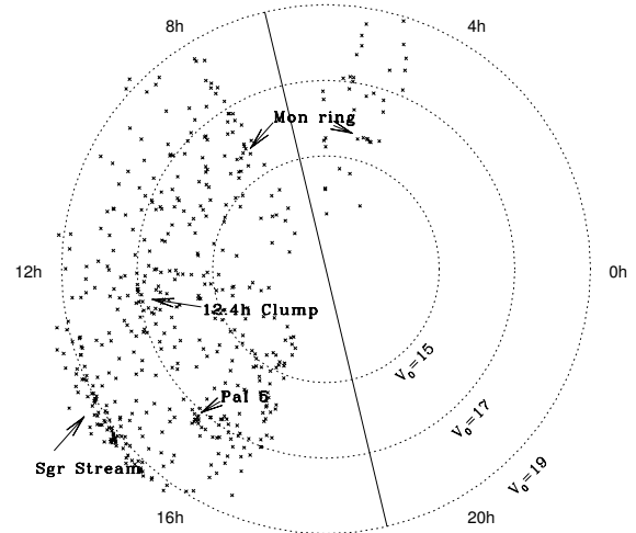
Fig. 2. Radial plot of the distribution of the 498 RR Lyrae stars in right ascension. The radial axis is the extinction corrected magnitudes, V_0 . The circles correspond to a distance from the Sun of 8, 19 and 49 kpc. The solid line indicates the position of the galactic plane.
