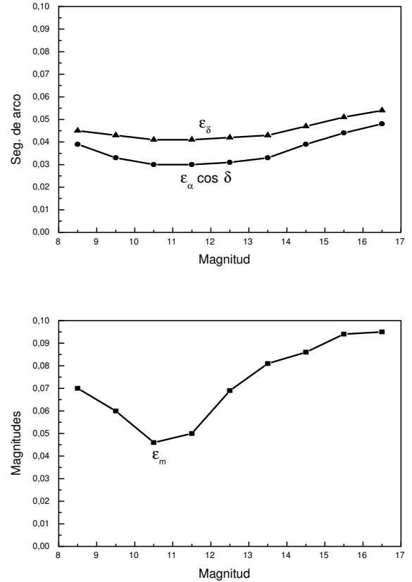
Fig. 1. Dependence on the average quadratic on magnitude.
