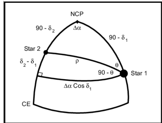
Fig. 1. The relation between (\rho, \theta) and (\alpha, \delta) coordinates.
