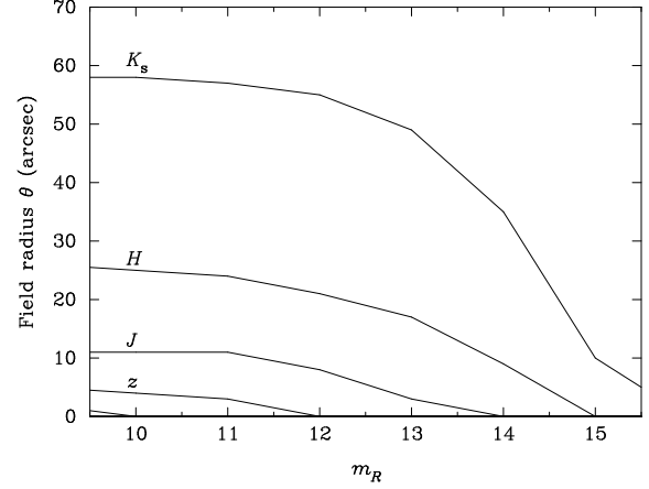
Fig. 6. The expected field radius \theta for a Strehl ratio of 0.25 against the guide star magnitude m_R in AO mode and in median conditions.
