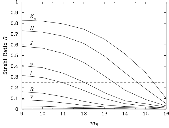
Fig. 4. The expected on-axis Strehl ratio R against the guide star magnitude m_R in AO mode and in median conditions. The dashed line marks the limit for good correction R \geq 0.25 .
