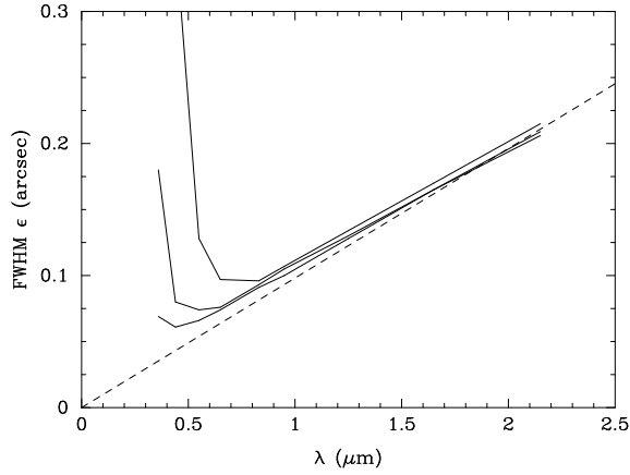
Fig. 2. The expected on-axis FWHM \epsilon with a magnitude 10 guide star in AO mode. The solid lines are the expected performance of Guieloa in first-quartile, median, and third-quartile conditions. The dashed line is the diffraction limit \lambda/D .
