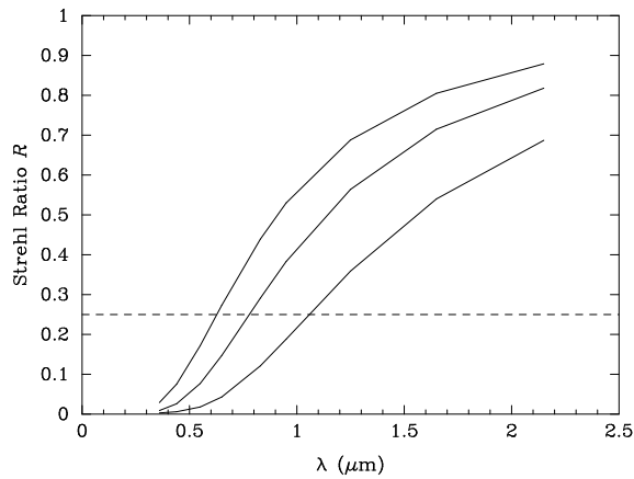
Fig. 3. The expected on-axis Strehl ratio R with a magnitude 10 guide star in AO mode. The solid lines are the expected performance of Guieloa in first-quartile, median, and third-quartile conditions. The dashed line marks the limit for good correction R \geq 0.25 .
