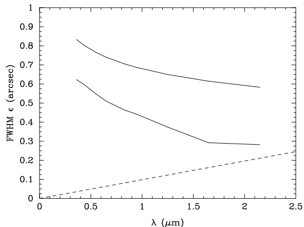
Fig. 8. The expected on-axis FWHM \epsilon in aO+FG mode with magnitude 14 and 16 guide stars in median conditions. The dashed line is the diffraction limit \lambda/D .
