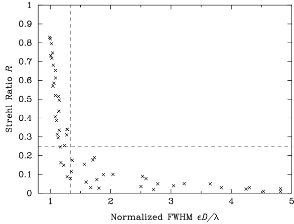
Fig. 5. The expected on-axis normalized FWHM \epsilon D/\lambda against the expected on-axis Strehl ratio R mode with guide stars between magnitudes 9 and 16 in AO mode and in median conditions. The dashed lines show the limits for good correction \epsilon \leq 1.33\lambda/D and R \geq 0.25 .
