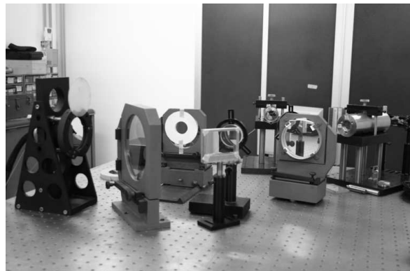
Fig. 1. Guieloa on an optical bench in the laboratories of the Instituto de Astronomía UNAM. The deformable mirror mounted on the articulated platform is at the far left. The wavefront sensor lens array is at the far right. The vibrating mylar mirror is the third component from the right.
