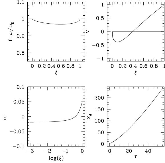
Fig. 5. Time dependent disk model.
