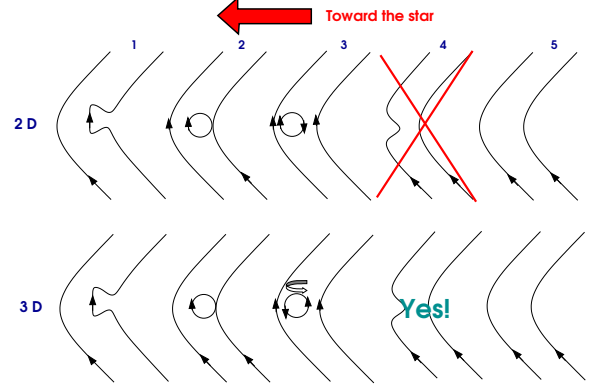
Fig. 3. Loop dynamics (S07).
