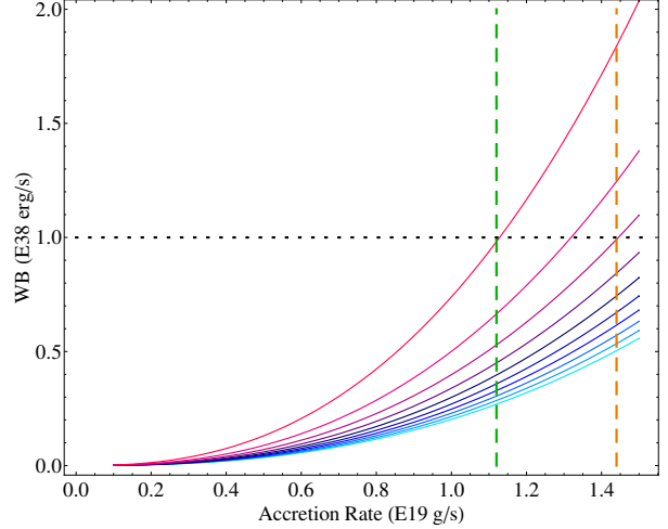
Fig. 1. Magnetic power released as function of mass accretion rate for different values of \beta (from blue to pink, \beta = 10 - 1 ). The black dotted line corresponds to the observed X-ray luminosity of GRS1915+105 microquasar. The green and orange vertical lines represent accretion rates of 80% and 100% the Eddington ones.
