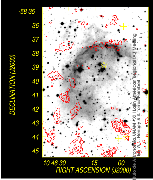
Fig. 1. Overlay of the DSS-R image of RCW 52 in grayscale and the continuum emission at 870\ \mu\text{m} in contours. Contours ranges from 20 to 50\ \text{mJy beam}^{-1} . The star, the square, and the crosses mark the position of IRAS, MSX, and 2MASS YSO candidates, respectively.
