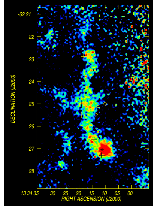
Fig. 2. Continuum emission at 870\ \mu\text{m} corresponding to one of the star forming regions in RCW 78. Colorscale ranges from 20 to 130\ \text{mJy beam}^{-1} . The star, the squares and the triangle, and the crosses mark the position of IRAS, MSX, and 2MASS YSO candidates, respectively.
