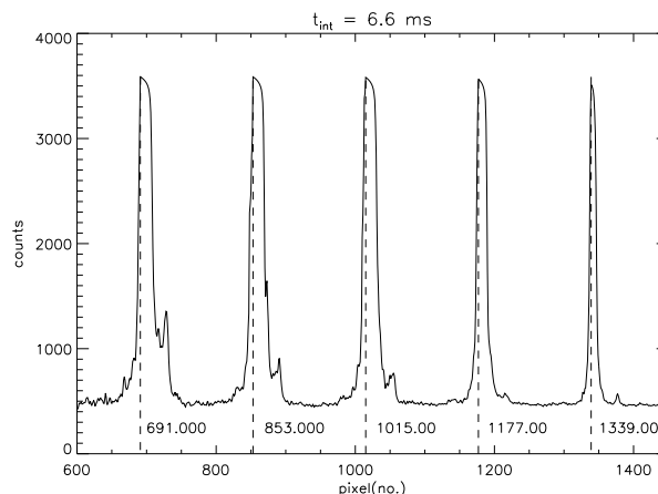
Fig. 1. Spectrum of the tested signal obtained with the acousto-optical cell. The dotted lines indicate the position of diffracted beam maximums on photo detector, the distance between these are equally spaced.
